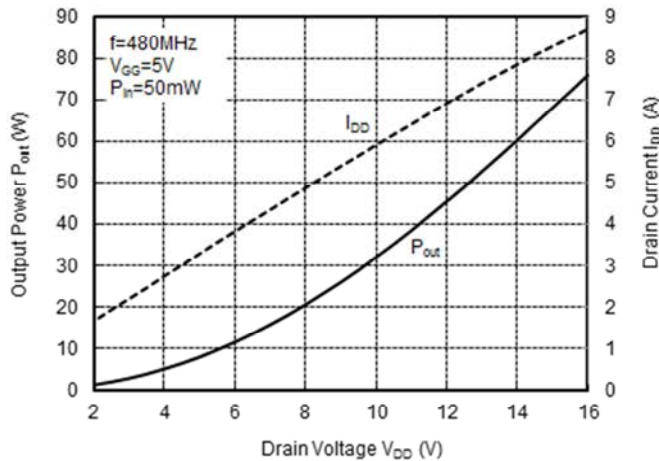
OUTPUT POWER, DRAIN CURRENT versus DRAIN VOLTAGE
