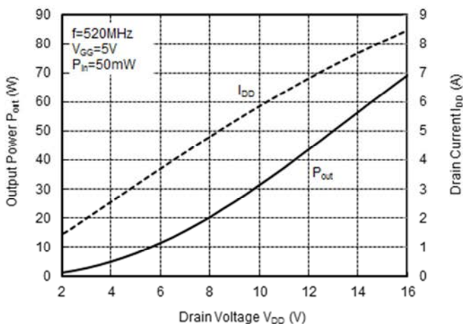
OUTPUT POWER versus DRAIN VOLTAGE
