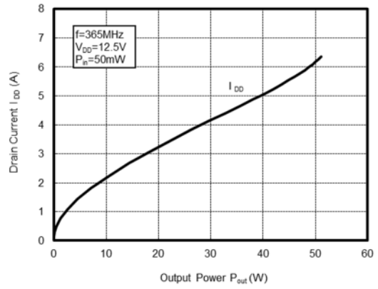
DRAIN CURRENT versus OUTPUT POWER
