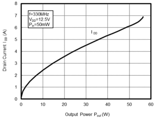
DRAIN CURRENT versus OUTPUT POWER
