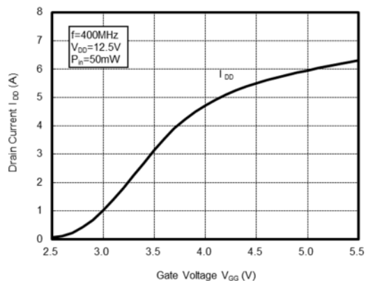
DRAIN CURRENT versus GATE VOLTAGE
