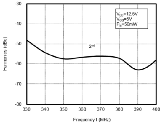
2 nd HARMONICS versus FREQUENCY
