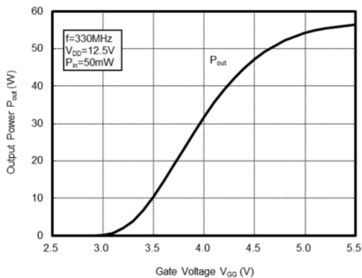
OUTPUT POWER versus GATE VOLTAGE
