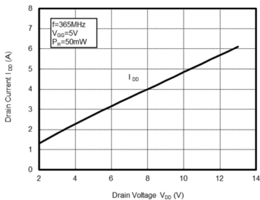
DRAIN CURRENT versus DRAIN VOLTAGE
