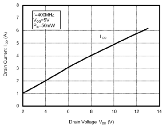
DRAIN CURRENT versus DRAIN VOLTAGE
