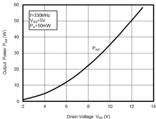
OUTPUT POWER versus DRAIN VOLTAGE
